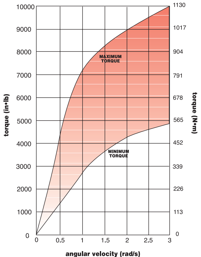
Typical Performance Curves FOR MODEL "SB" SHOCK ABSORBERS
