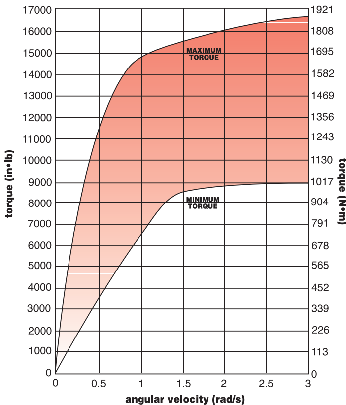
Typical Performance Curves FOR MODEL "RC" SHOCK ABSORBERS
