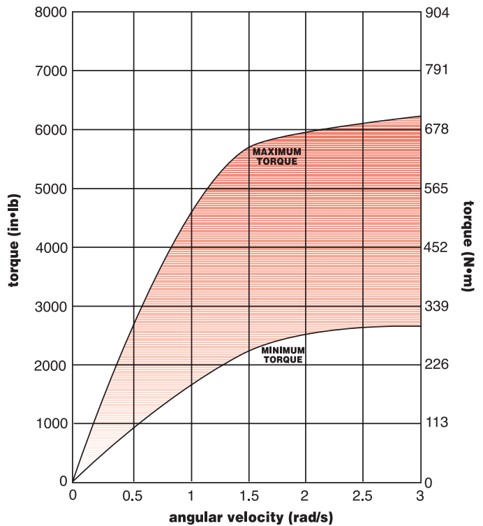
Typical Performance Curves FOR MODEL "H" SHOCK ABSORBERS
